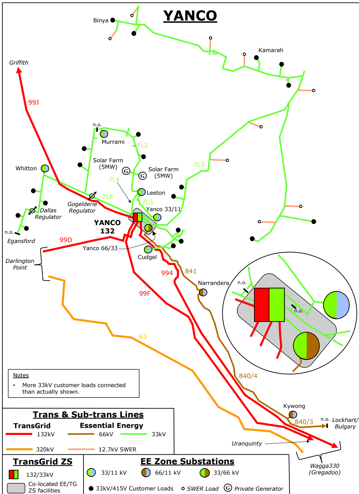
Sub-transmission Single Line Diagram of Yanco area
