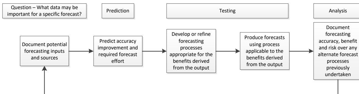
Figure 4 – Forecasting Methodology
